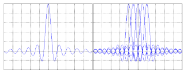
Figure 1: Spectra of (a) an OFDM sub-channel and (b) an OFDM signal.
