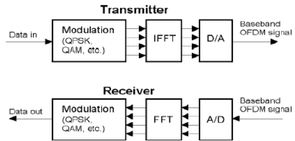
Figure 2: Basic FFT, OFDM transmitter and receiver
